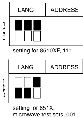
Figure 7. Synthesizer dip switch language settings
