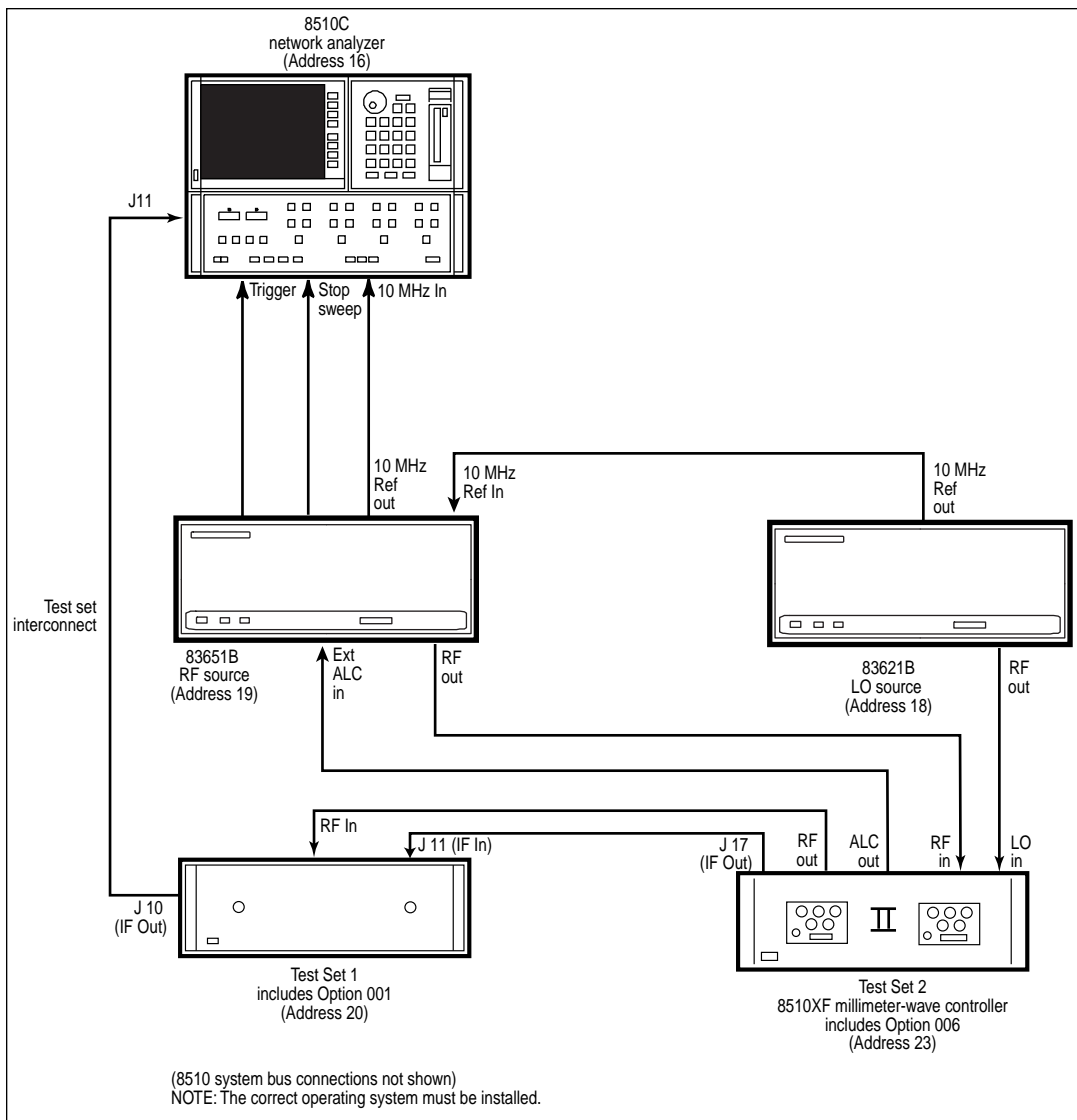
Figure 8. Agilent 8510XF system configured with a microwave test set (simplified)
