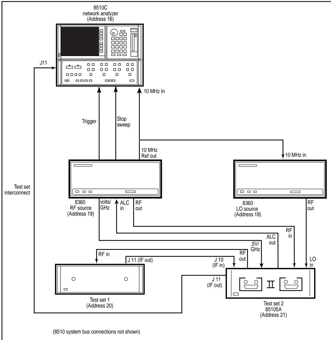
Figure 5. Dual test set configuration with millimeter-wave and microwave test sets (simplified)
